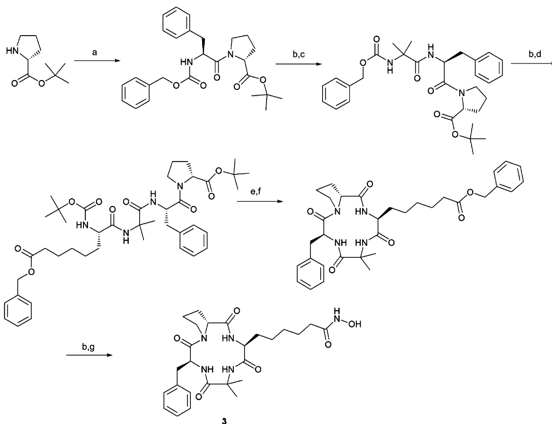
Scheme 1. Synthesis of cyclic tetrapeptide. Reagents and conditions: (a) HBTU, DIEA, Z-L-Phe; (b) Pd–C, H 2 ; (c) HBTU, DIEA, Z-Aib; (d) HBTU, DIEA, Boc-L-Asu(OBzl); (e) TFA; (f) HATU, DIEA; (g) NH 2 OH, BOP, HOBT.
