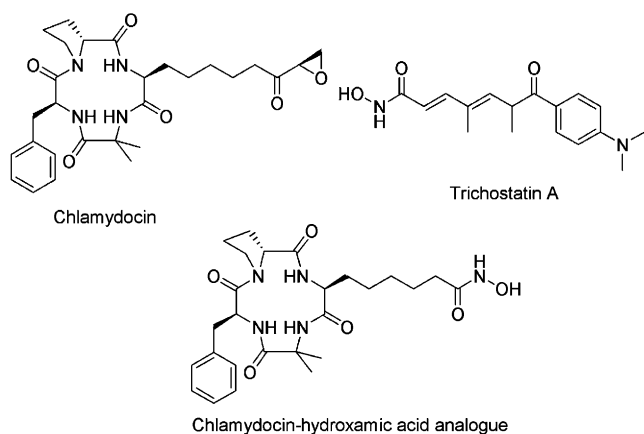
Figure 1. The structure of chlamydocin, trichostatin A, and proposed chlamydocin–hydroxamic acid analogue.
