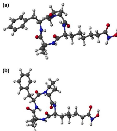
Figure 3. Energy minimized structures of the two conformers of chlamydocin–hydroxamic acid analogue: (a) bis- \gamma -turn and (b) \beta -turn.
