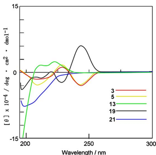
Figure 2. CD spectra of chlamydocin–hydroxamic acid analogues.
